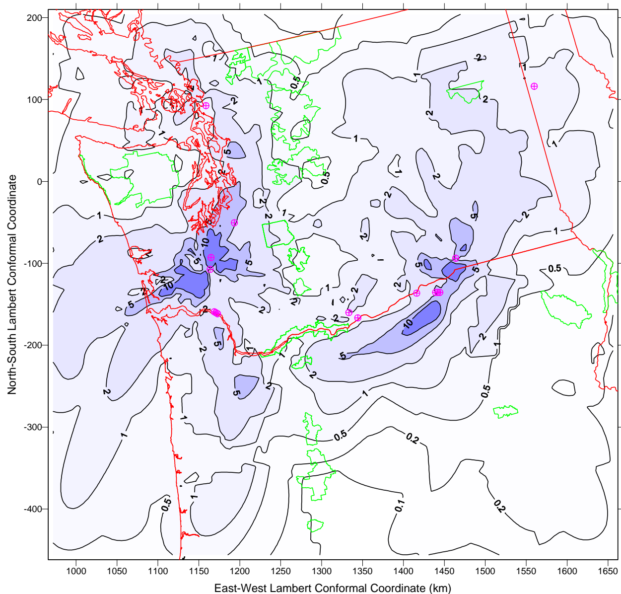
Figure 3. Maximum 24-hour Extinction Coefficient (1/Mm) at Each Receptor Based on a Winter Simulation of Baseline Sources (Oil-Fired) 5 Plus the Wallula Power Project
