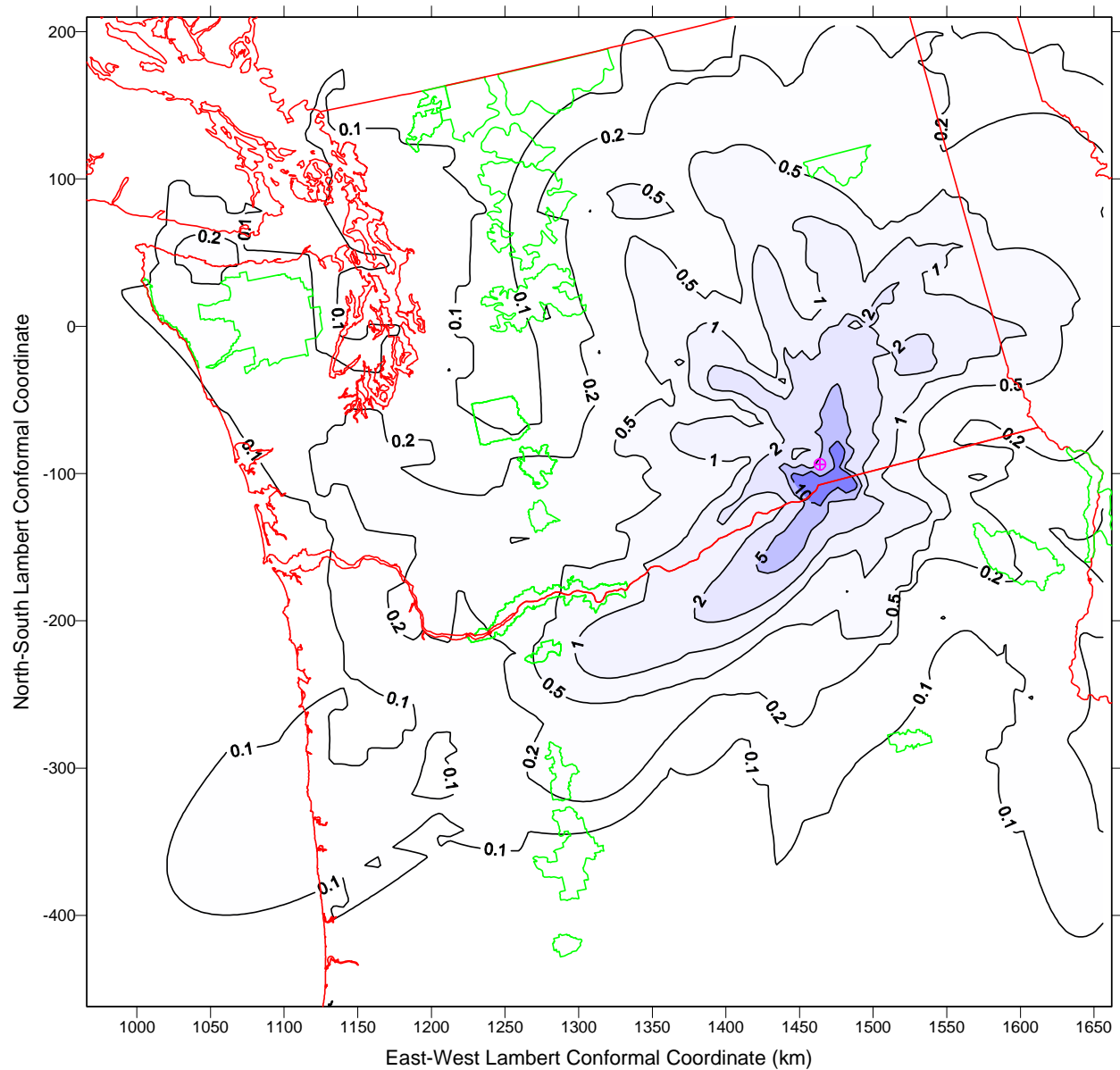
Figure 4. Maximum 24-hour Extinction Coefficient (1/Mm) at Each Receptor Based on an Annual Simulation of the Wallula Power Project Alone
