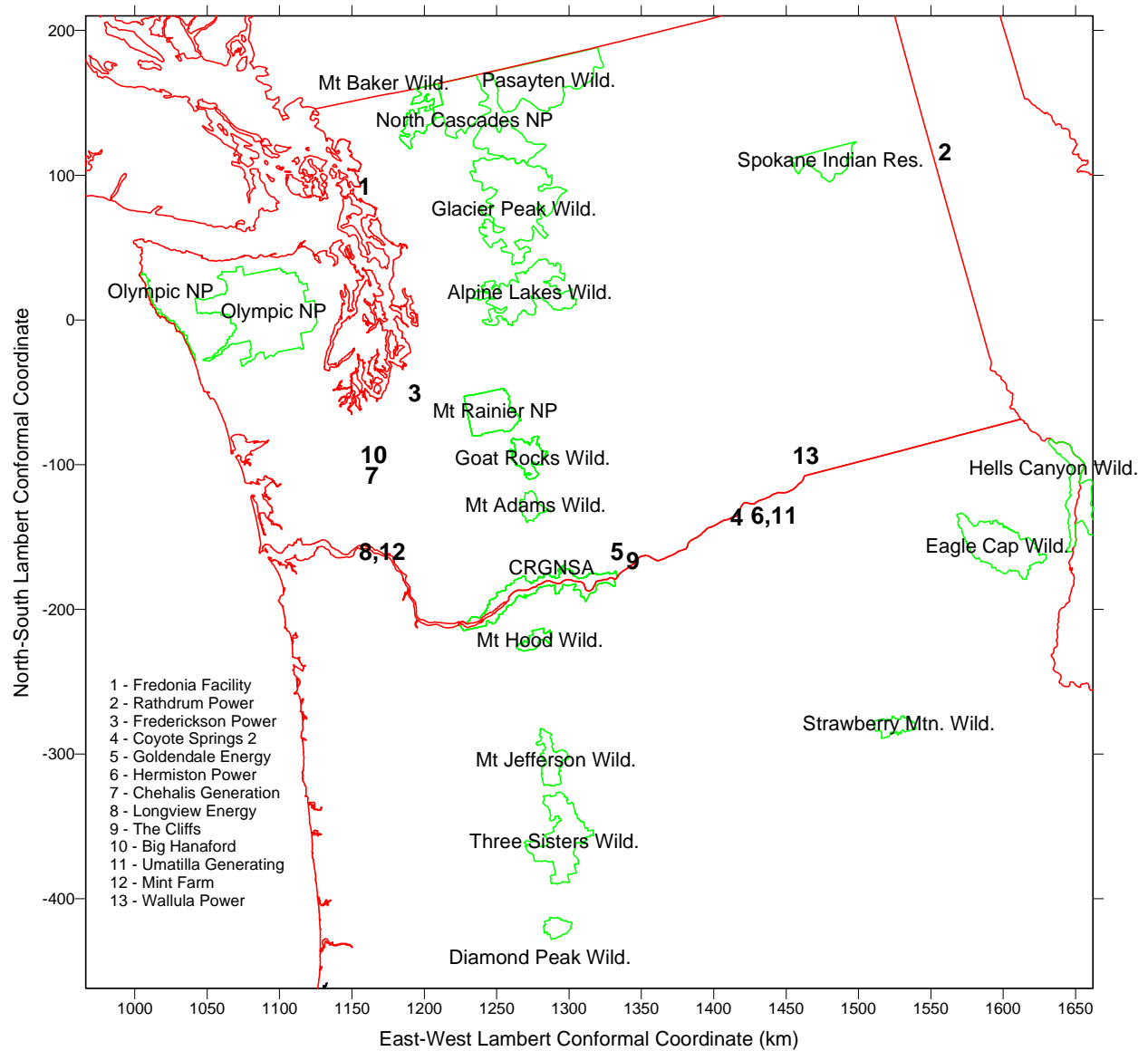
Figure 1. Baseline Sources with Wallula Power Project
