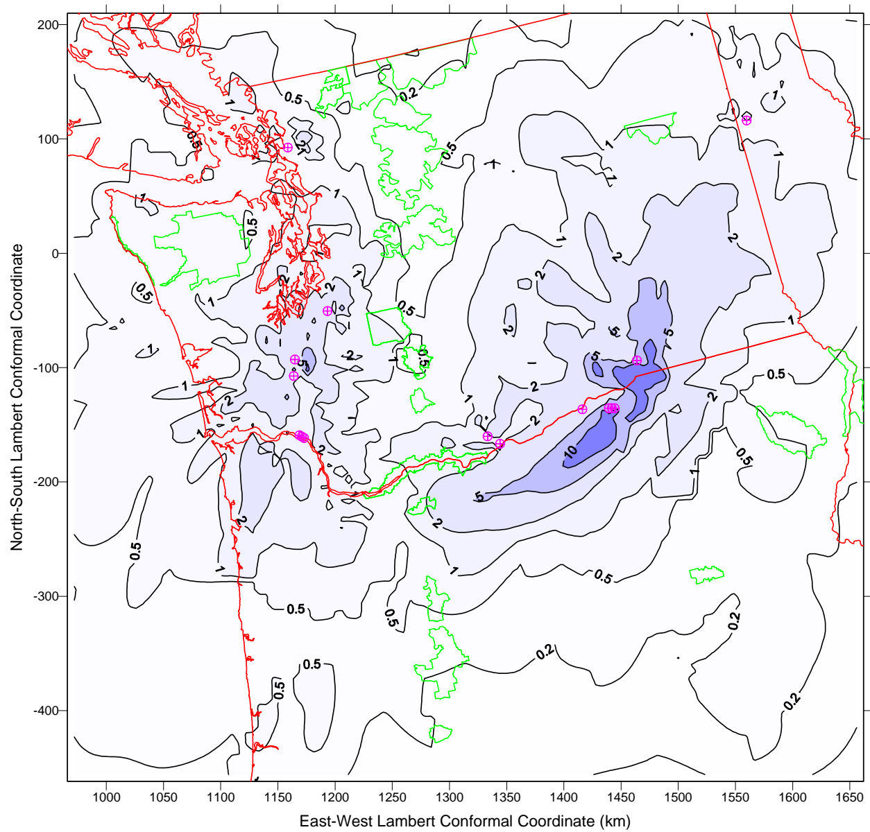
Figure 2. Maximum 24-hour Extinction Coefficient (1/Mm) at Each Receptor Based on an Annual Simulation of the Baseline Sources (Gas-fired) Plus the Wallula Power Project
